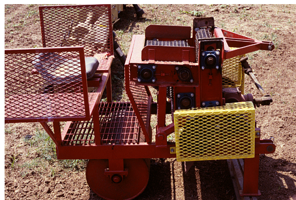
Sprig Planters
