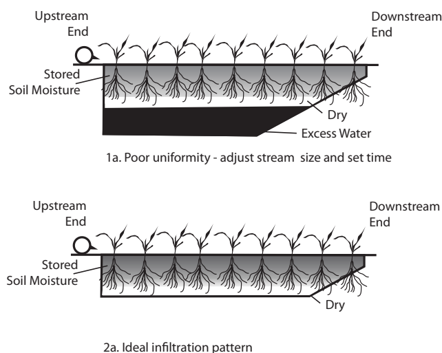
Figure 1. Infiltration profiles under conventional furrow irrigation.
