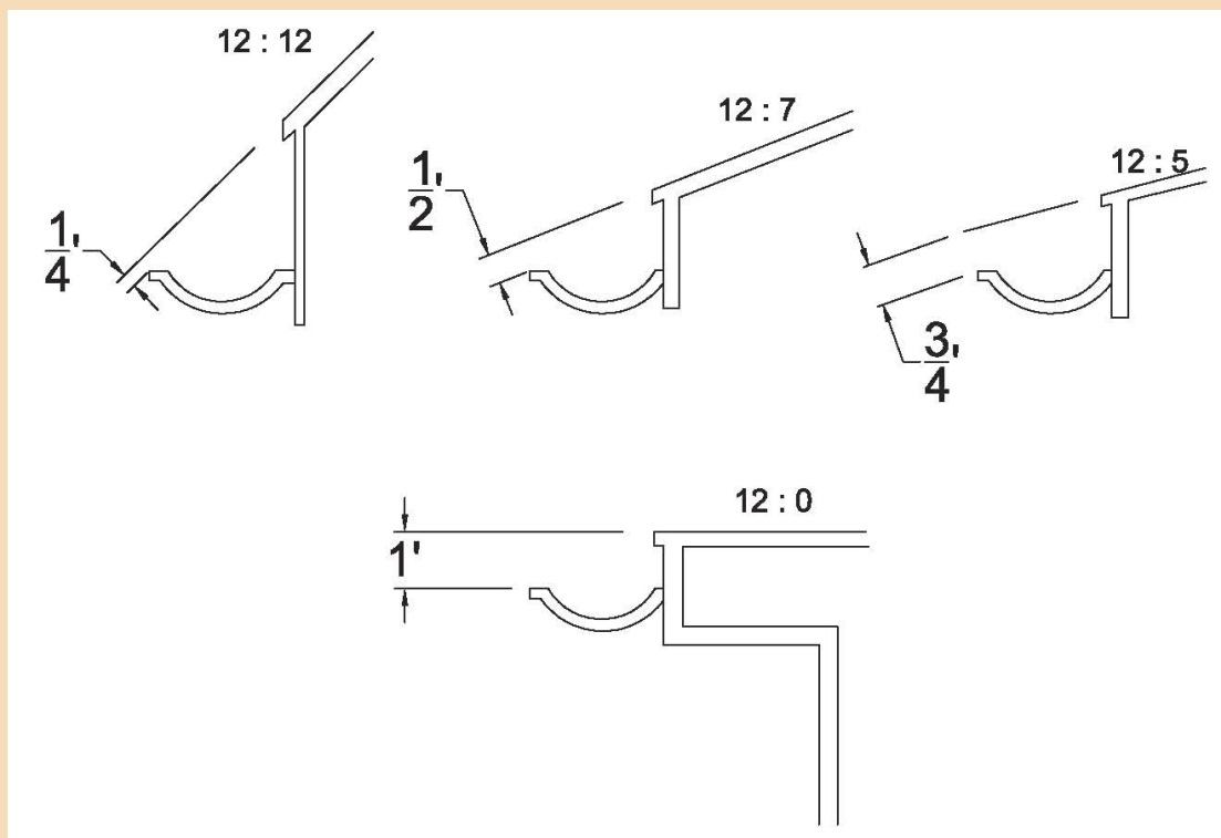
Figure 3. Properly position gutters. Snow and ice can slide off the roof clear of the gutter. Steeper pitch roofs require less clearance.
