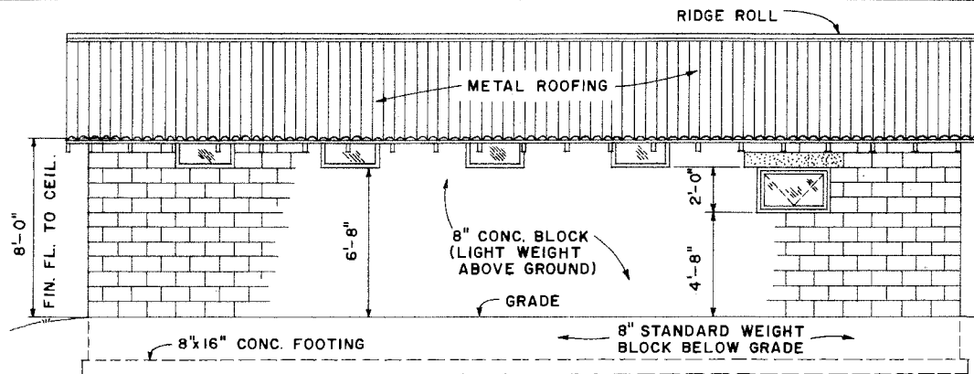
SIDE ELEVATION
