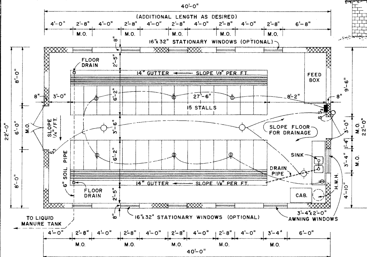
FLOOR PLAN
