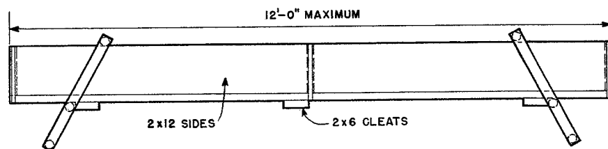
SIDE ELEVATION
