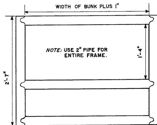
SUPPORT FRAME
