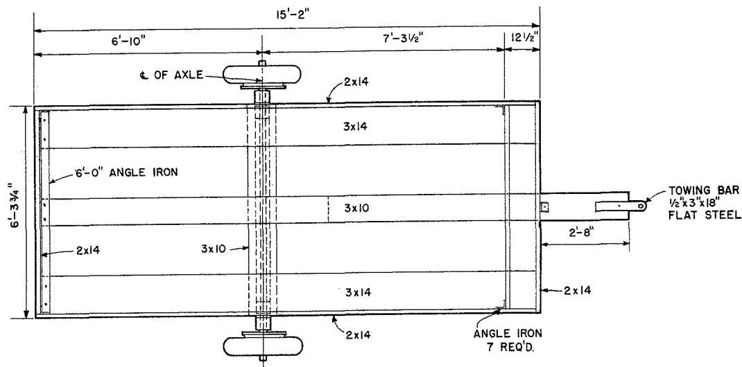
TOP VIEW OF BED FRAME
