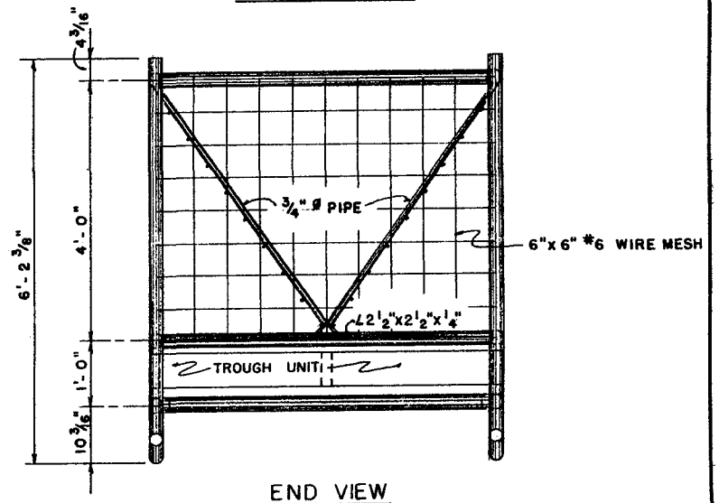
TROUGH UNIT
