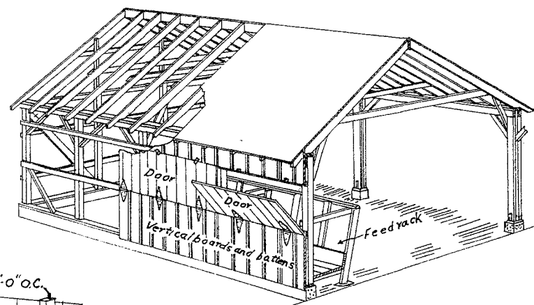
PART FRAMING ELEVATION
