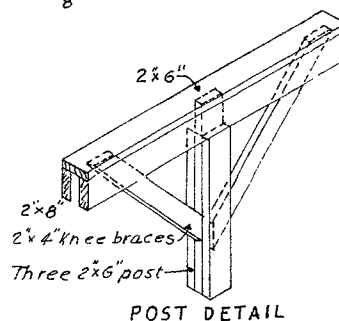
POST DETAIL
