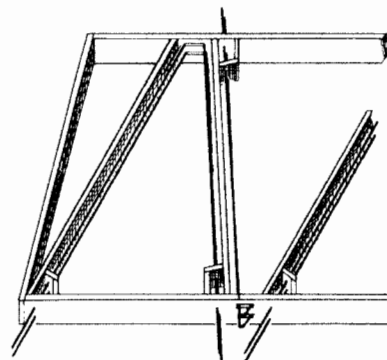
3 VIEW SHOWING REINFORCING BUTTRESS BARS B, IN PLACE.
