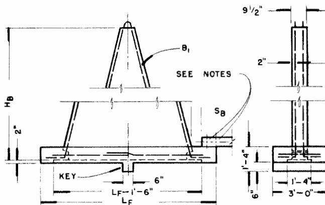
SIDE VIEW of BUTTRESS SCALE: 3/8" = 1' 0"
