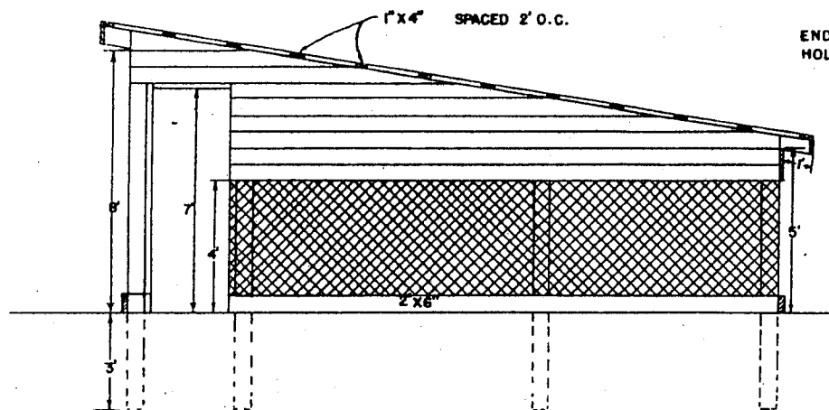
SCALE 3/8" = 1'-0"
