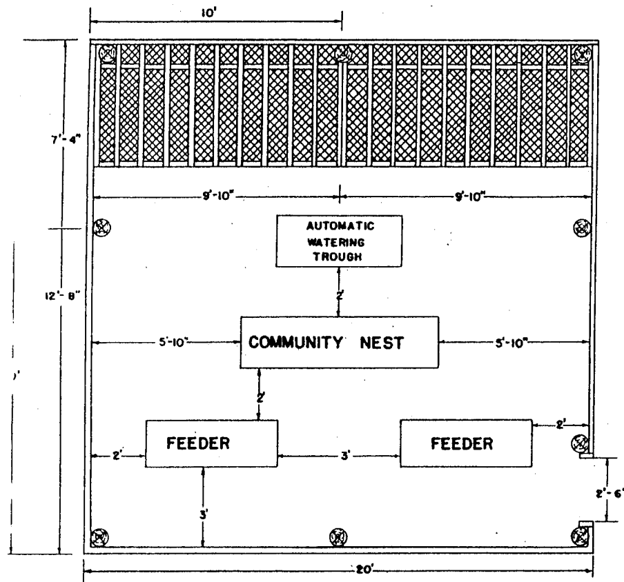
SCALE 3/8" = 1'-0"
