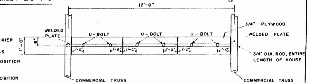
PLAN VIEW OF BAFFLE
