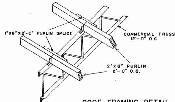
ROOF FRAMING DETAIL
