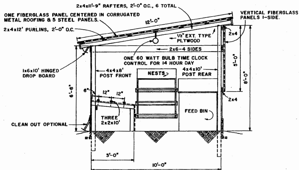
ALTERNATE ROOF & LAYOUT
