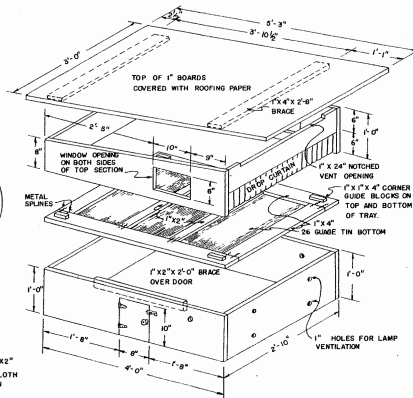
ISOMETRIC OF LAMP BROODER SCALE: 1" = 1'-0"
