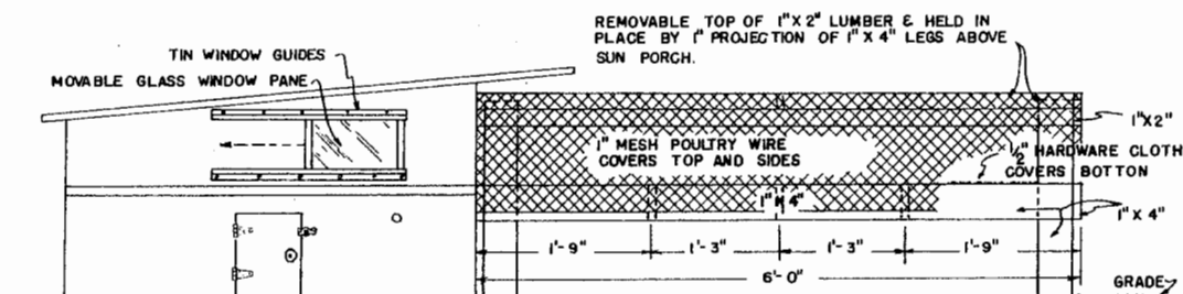
LAMP BROODER AND SUN PORCH
