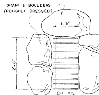
PLAN SIMPLE LOW-COST FIREPLACE
