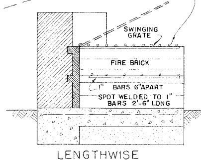
LENGTHWISE
