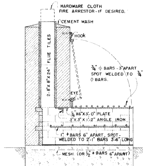
LENGTHWISE SECTION FIREPLACE
