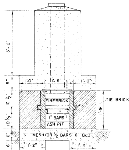
CROSS SECTION FIREPLACE WITH CHIMNEY
