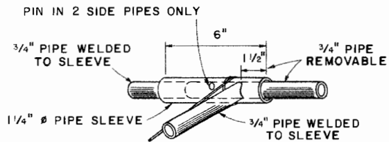
DETAIL "B"
