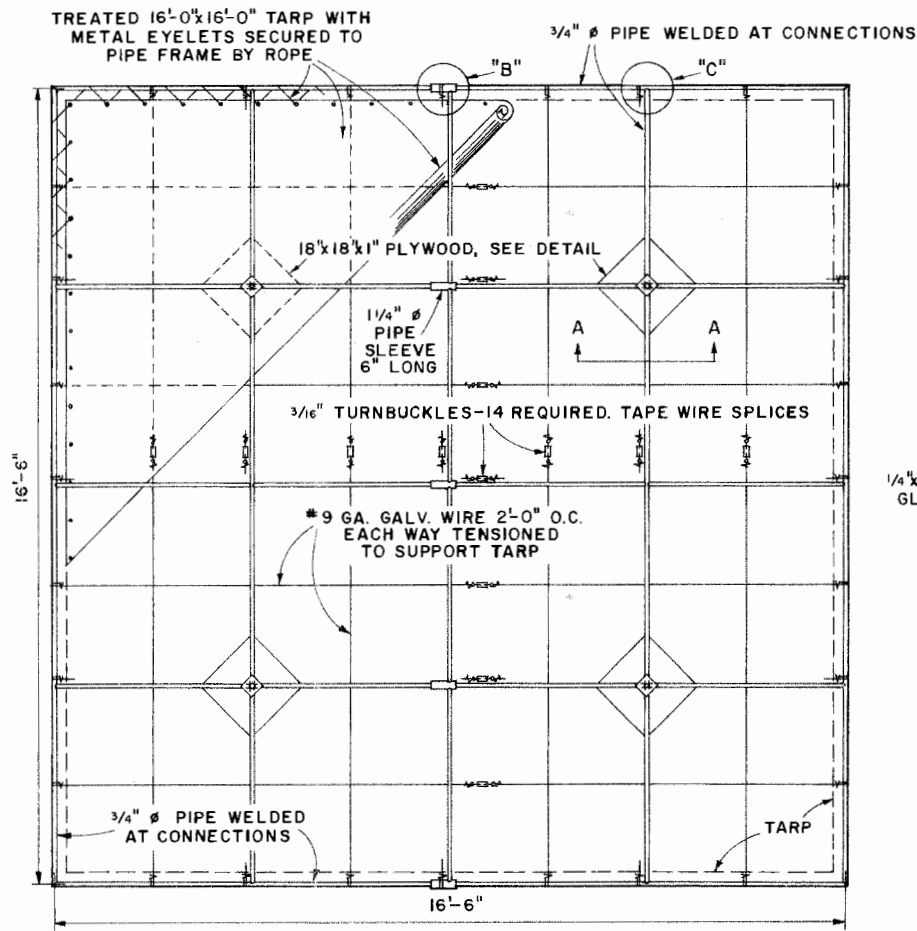
PLAN OF FRAME
