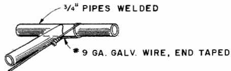
DETAIL "C"
