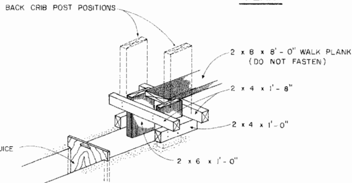
WALK PLANK SUPPORT DETAIL
