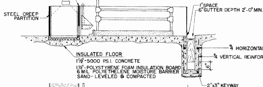
TIED FARROWING STALL WITH DEEP NARROW GUTTER SEE NOTES: 1,2,4,6,8,10,11.
