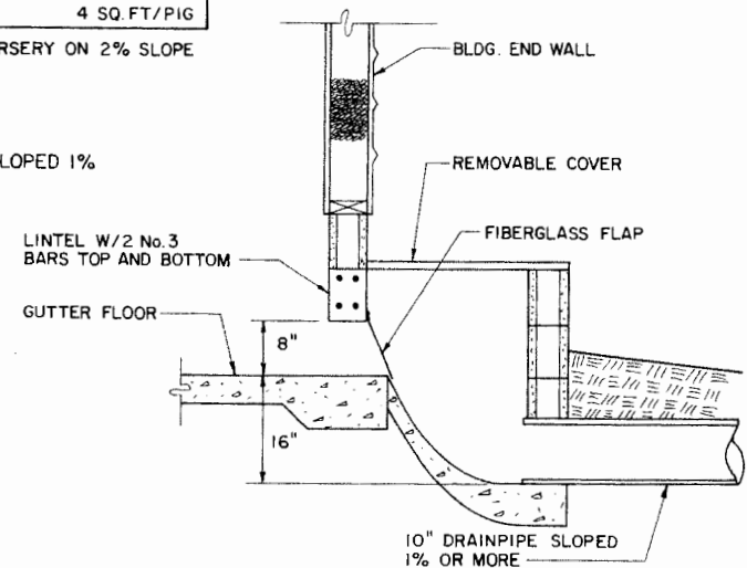
GUTTER DRAIN DETAIL NOT TO SCALE
