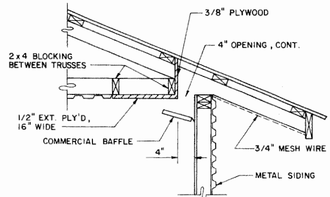
AIR INLET DETAIL NOT TO SCALE
