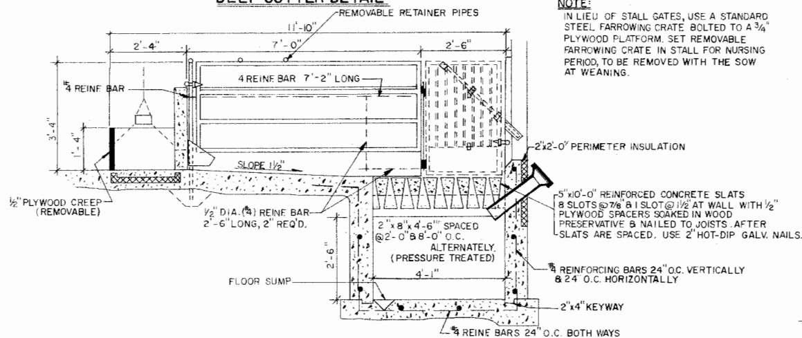
SLOTTED FLOOR DETAIL
