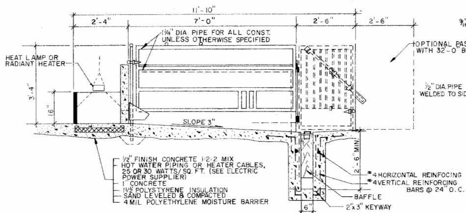
DEEP GUTTER DETAIL
