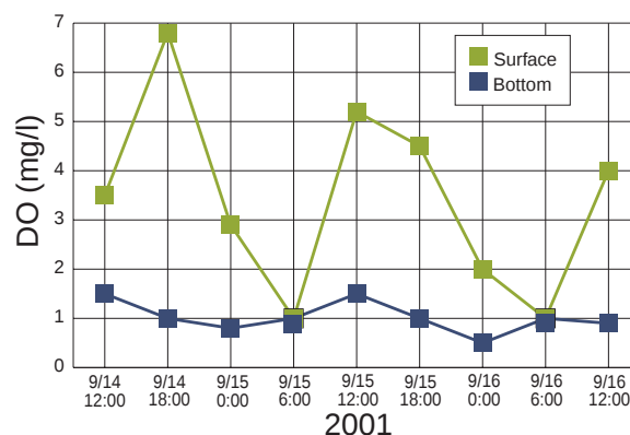
Figure 3. Dissolved oxygen concentrations recorded at the surface and bottom (1 m depth) of a hydrilla bed in the Atchafalaya Basin during September 2001. Note the continual hypoxic conditions on the bottom and the nocturnal hypoxia at the surface.
