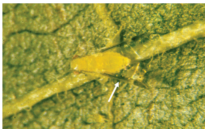
Figure 3. Blackmargined aphid.
