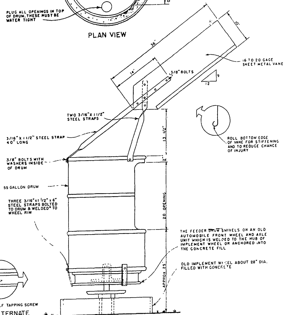
SIDE ELEVATION
