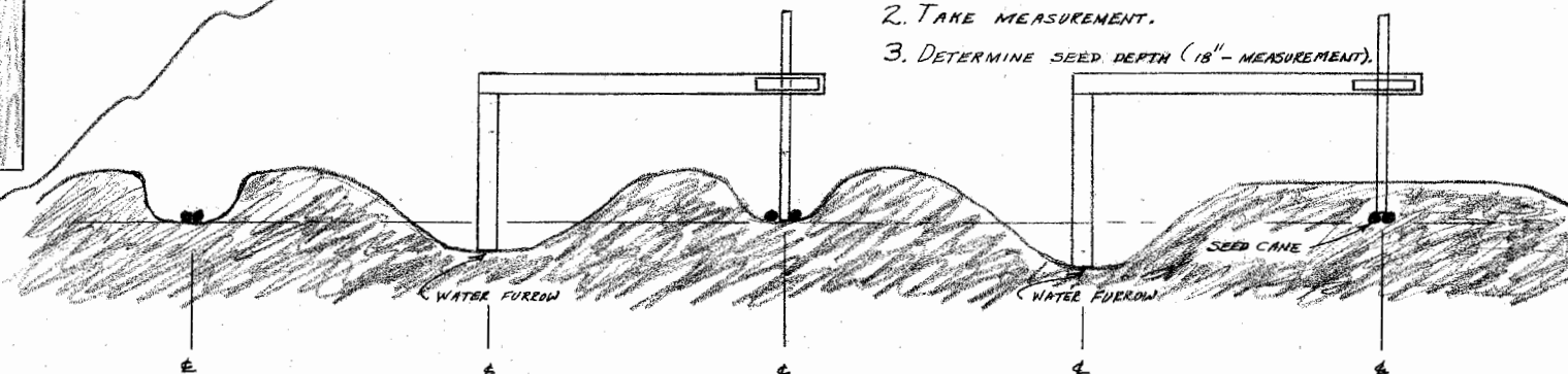
CROSS SECTION OF CANE ROWS
