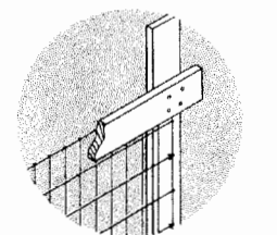
GATE PANEL DETAIL
