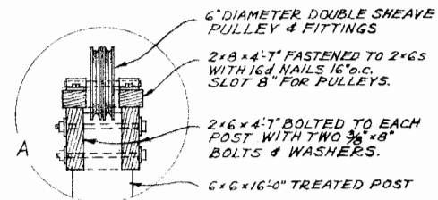
PULLEY & BEAM DETAIL SCALE: 1\frac{1}{2}" = 1'-0"
