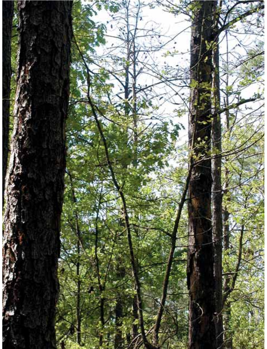
Many of the forests that once grew longleaf pine are now growing loblolly, which is showing signs of decline. The loblolly pine in the center of this Alabama forest shows signs of disease.
