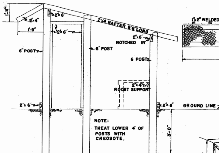
FRAMING SECTION
