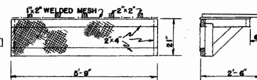
ROOST DETAIL
