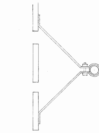
STATIONARY PIPE FENDER
