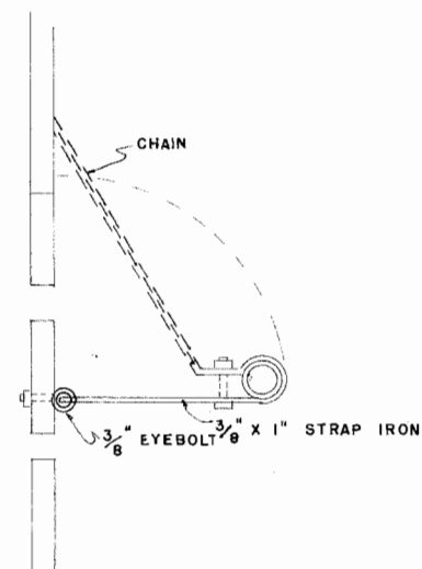
FOLDING PIPE FENDER
