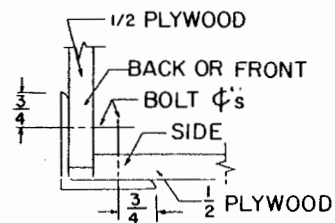
CORNER DETAILS SCALE: 1/2"=1"
