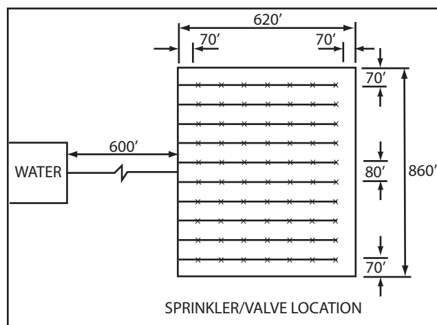
Figure 17. Schematic layout of a permanent irrigation system used to apply animal waste.
