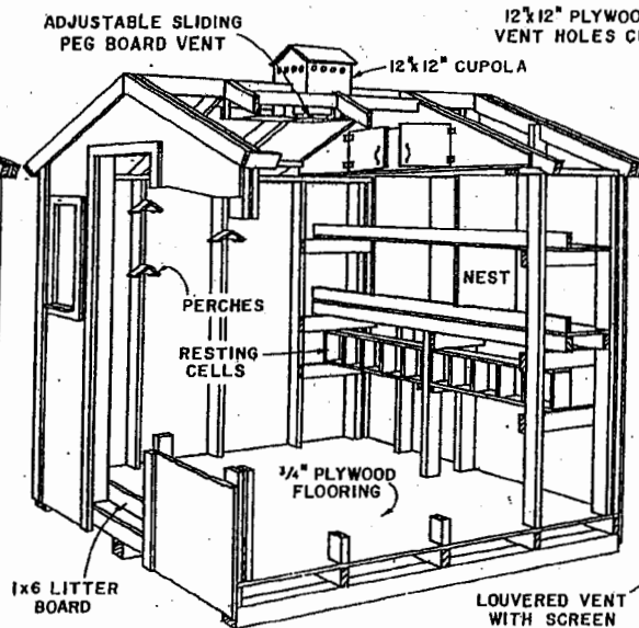
PERSPECTIVE OF PIGEON HOUSE
