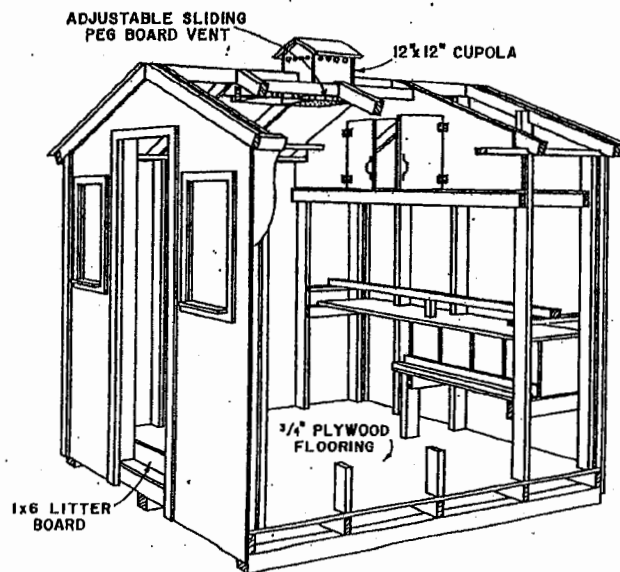
CUTAWAY VIEW OF 8x8' LAYING HOUSE
