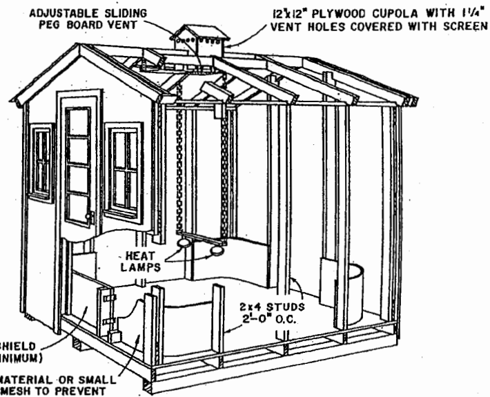
CUTAWAY VIEW OF 8x8' BROODER HOUSE
