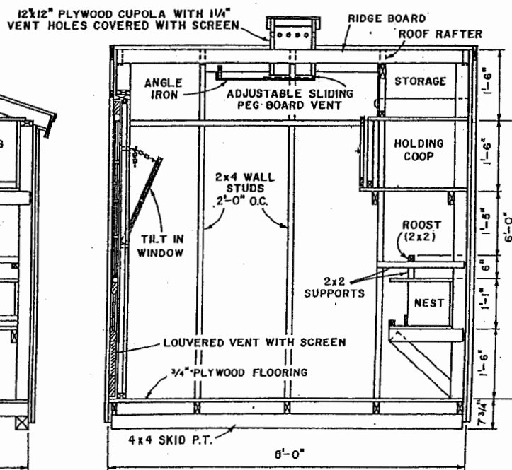
SECTIONS OF CHICKEN HOUSE-BANTAMS
