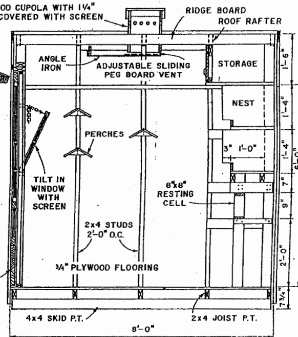
SECTION OF PIGEON HOUSE
