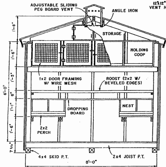
SECTIONS OF CHICKEN HOUSE-BANTAMS
