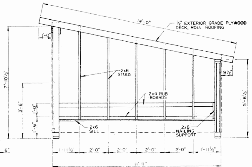
SIDE VIEW
