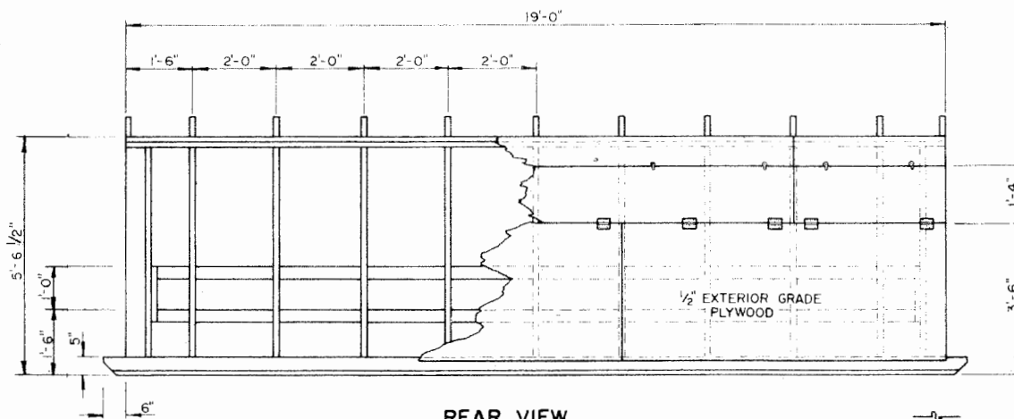
REAR VIEW
