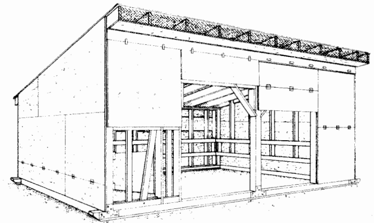
PERSPECTIVE
