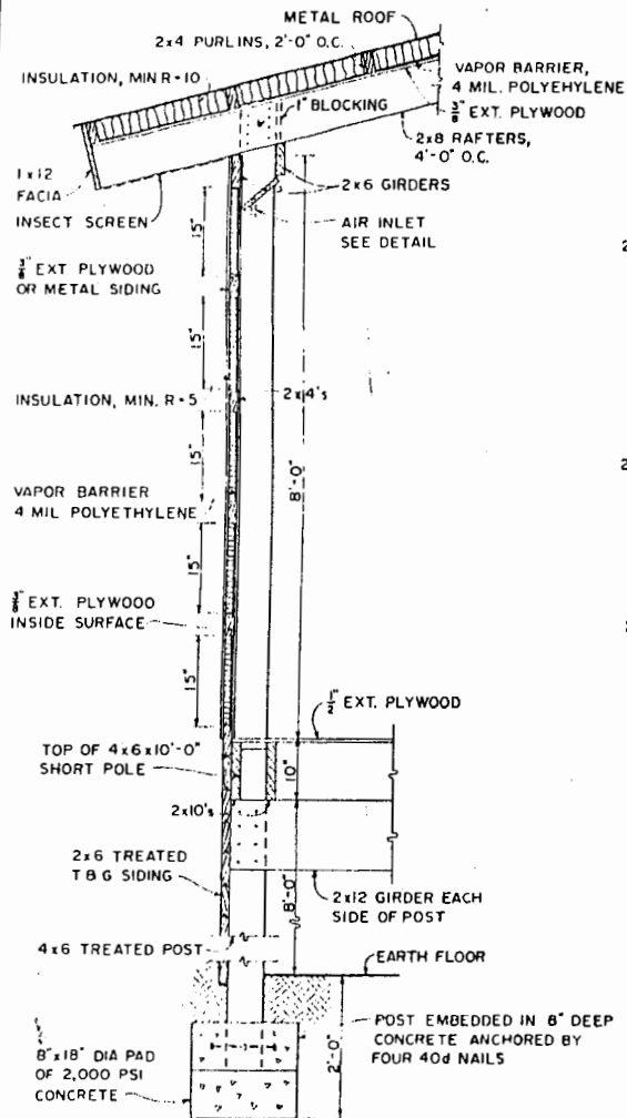
WALL SECTION A-A
