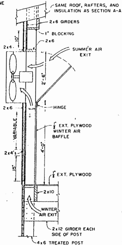
WALL SECTION B-B OF FAN DETAIL
