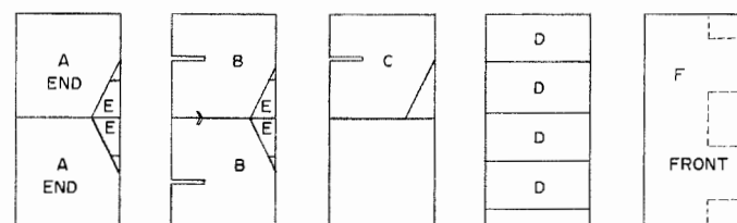
PLYWOOD CUTTING DIAGRAM SCALE: 1/4"=1'-0"
