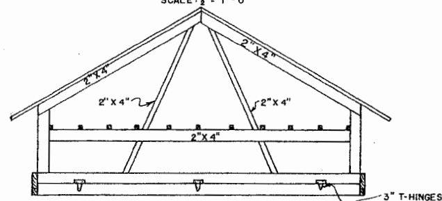
REAR VIEW SCALE: \frac{1}{2} " = 1'-0"
