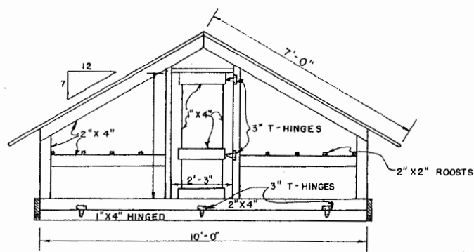
FRONT VIEW SCALE: \frac{1}{2} " = 1'-0"
