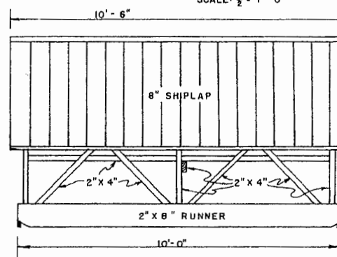
SIDE ELEVATION SCALE: \frac{1}{2} " = 1'-0"
