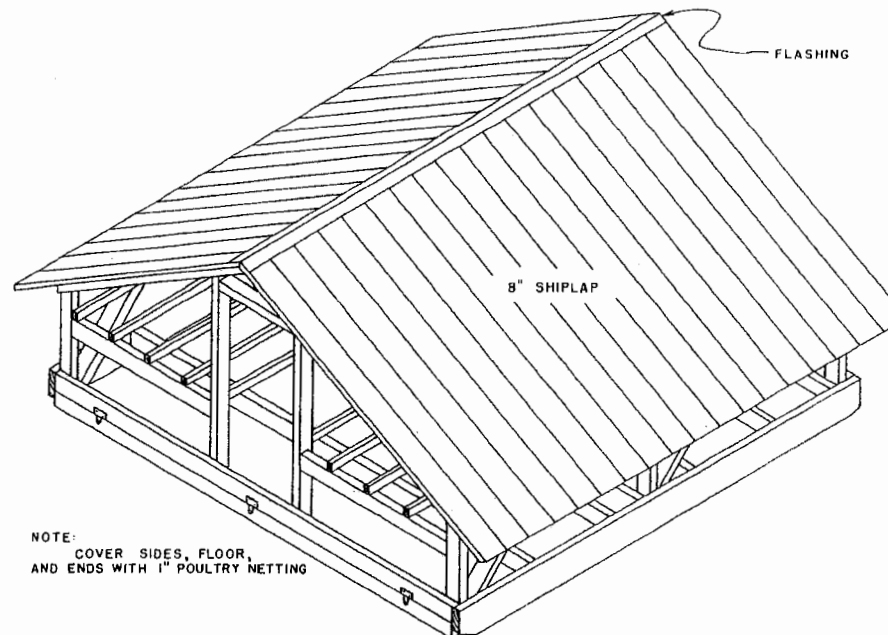
ISOMETRIC VIEW SCALE: \frac{1}{2} " = 1'-0"
