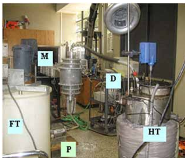
Figure 2. Schematic design (left) and actual set-up of the pilot scale continuous microwave assisted extraction system (right). T1-T4 indicates the thermocouple locations along the process line, M- microwave, P-pump, FT- feed tank, HT- holding tank, D- data acquisition system.
